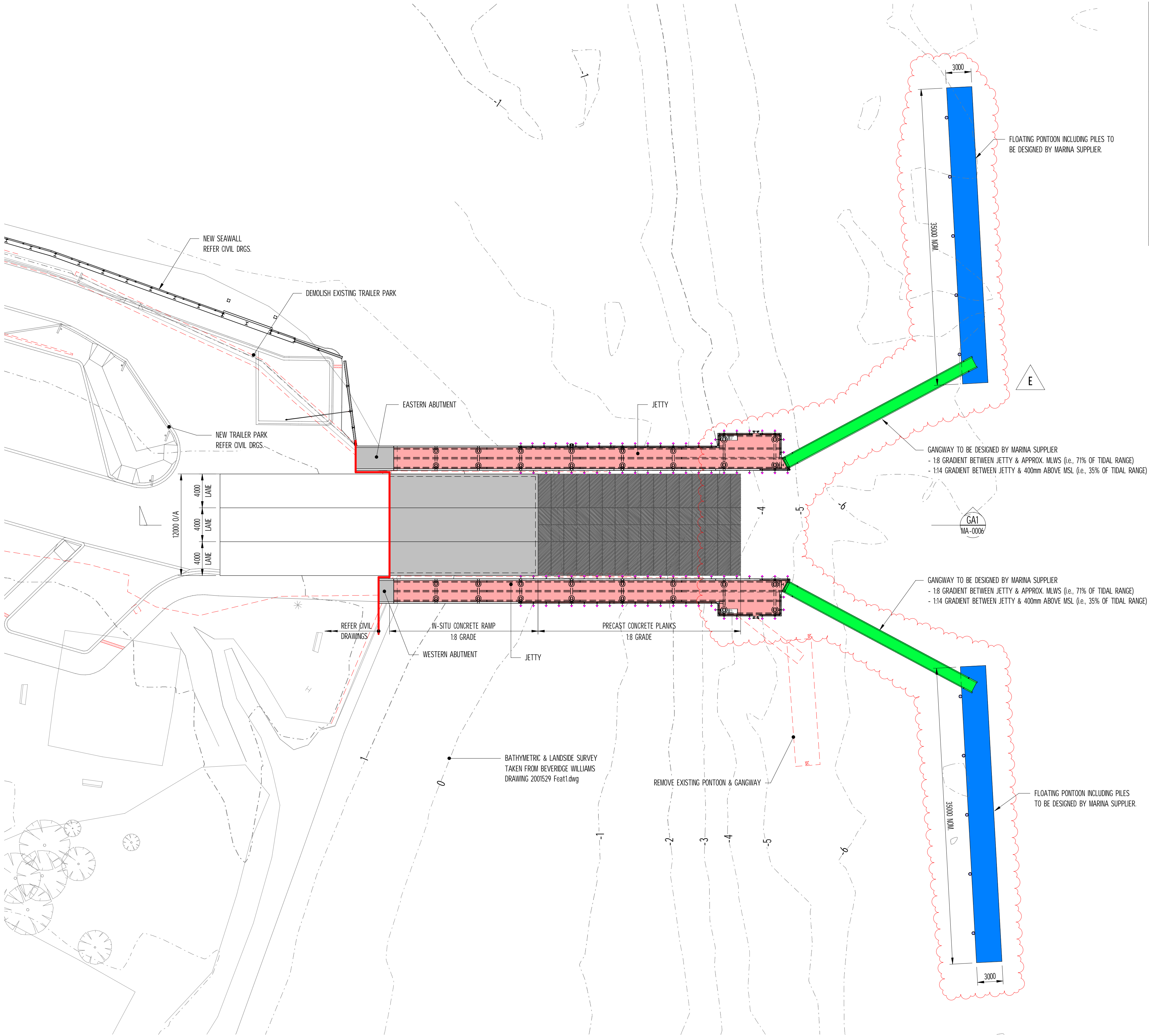
GENERAL ARRANGEMENT PLAN
